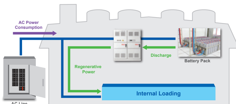
Regenerative function
